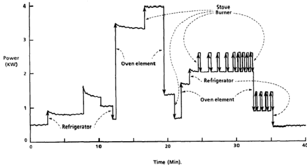
Figure 5: “Power v. time (total load) shows step changes due to individual appliance events.” 131
